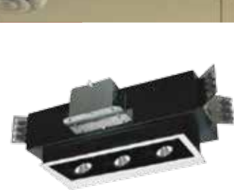
Multiple Cluster
