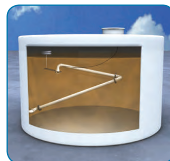
766: Scissor-style for large vertical tanks.
