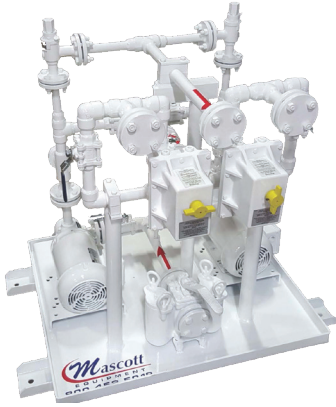
MASCOTT DUPLEX PUMP SKIDS
