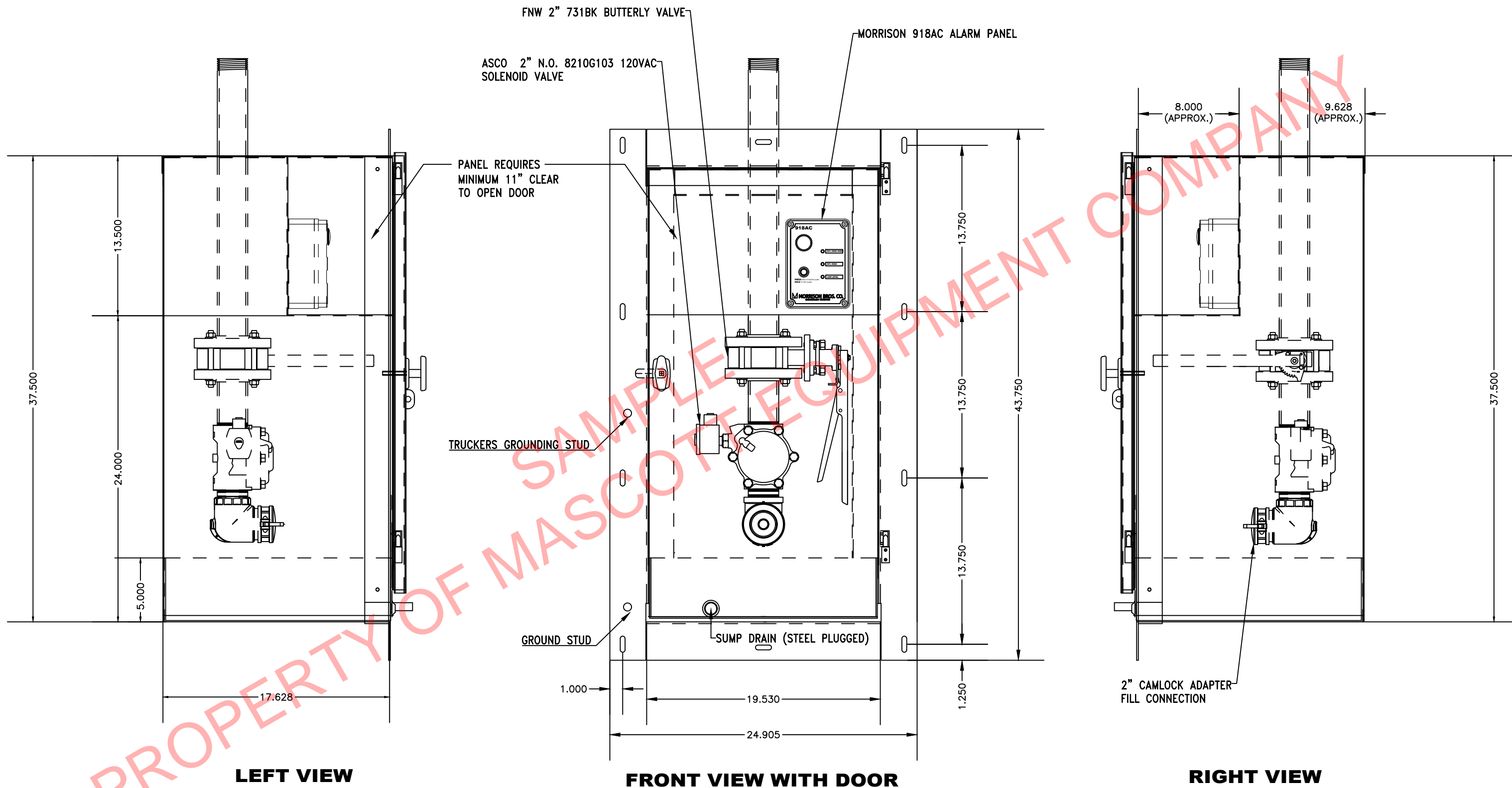
OUTLINE_DRAWING
