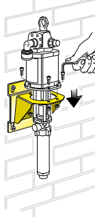
Art. 10/12 Wall bracket in painted steel for wall-mounting of divorced industrial pumps, series 900 and 1200
